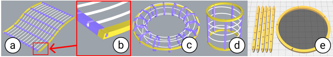
Fig. 15. Filament wiring system. (a) The script creates frames using the UV mapping of a selected surface, and (b) the filament can be fixed to the frames once connected. (c) According to the geometry of a surface, the system adjusts the number of frames. For example, in the torus, one yellow frame is needed because its edges are closed in the U and V directions. (d) When the edge is closed, users can select a one-stroke (spiral) path of the filament. (e) Using a conventional slicer (e.g., Ultimaker Cura), the frames can be printed.
