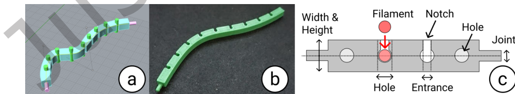
Fig. 11. Frame design script creates (a) a frame with the parameters(c) and (b) the frame can be 3D printed.
