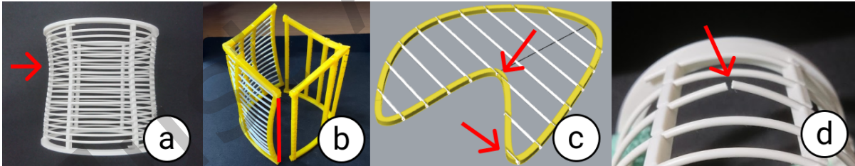
Fig. 16. Limitations of our techniques. (a, b) By wiring tightly, the frames deform as if pulled by the filament. (c) Paths of the filament is not uniquely determined for an arbitrarily shaped surface. (d) Filaments, especially in the case of PLA, may be broken during wiring.
